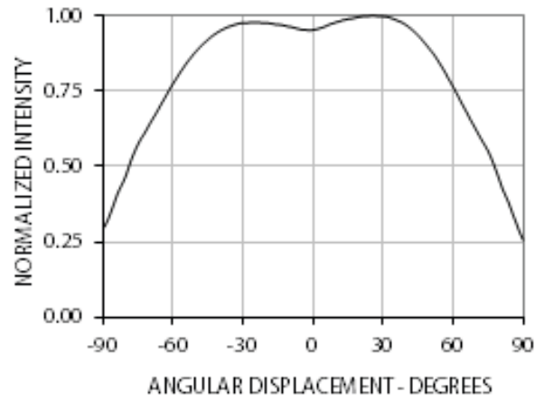
Figure 8 Radiation Pattern
